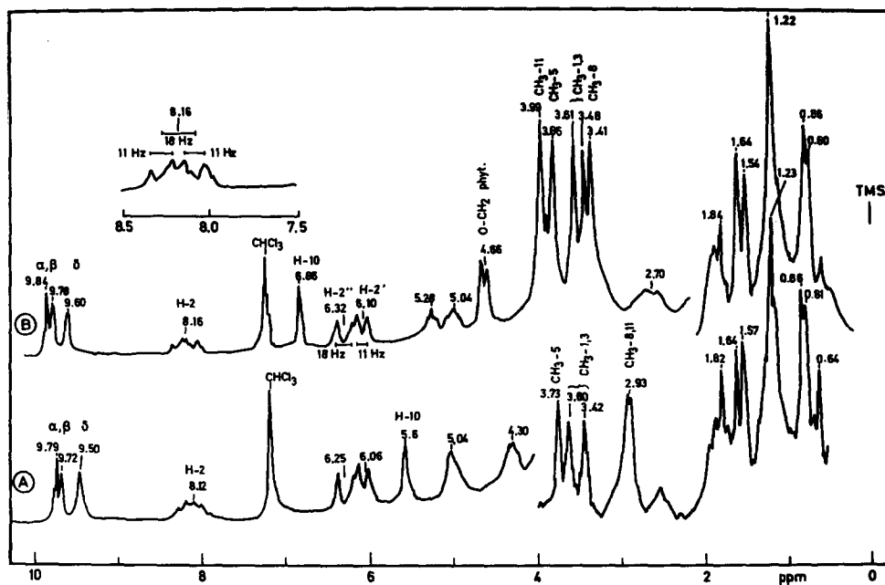
Fig. 4. ^1\text{H} magnetic resonance spectra at 100 MHz for anhydrous PChI-a ( 3.5 \cdot 10^{-2} M) in dry \text{C}_2\text{HCl}_3 (curve A) and in 0.5 % \text{C}_2\text{H}_3\text{O}_2\text{H}/\text{C}_2\text{HCl}_3 (curve B).
