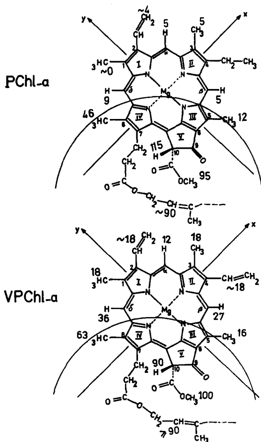
Fig. 10. Aggregation maps of PChl- a and VPChl- a . The shift differences (in Hz) between dimer ( C^2HCl_3 ) and monomer (0.5% C^2H_3O^2H/C^2HCl_3 ) are indicated for the individual protons. The semi-circle indicates the area of maximum interaction in the dimer.
