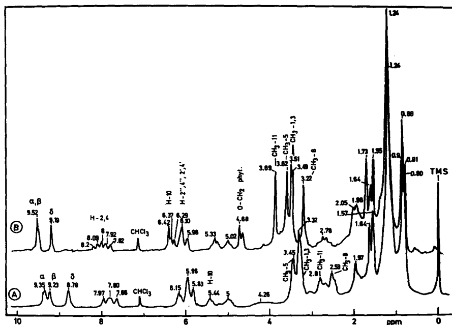
Fig. 5. ^1\text{H} magnetic resonance spectra at 90 MHz for anhydrous VPChI-a ( 5 \cdot 10^{-2} M) in dry \text{C}_2\text{HCl}_3 (curve A) and in 0.5 % \text{C}_2\text{H}_3\text{O}_2\text{H}/\text{C}_2\text{HCl}_3 (curve B).
