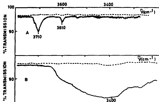
Fig. 1. Infrared spectra in the 3000–3800 \text{cm}^{-1} region (IRTRAN cell; 2 mm pathlength). (A) ---, anhydrous \text{CCl}_4 ; —, water-saturated \text{CCl}_4 ; (B) ---, anhydrous PChl- a ( 3 \cdot 10^{-2} M) in dry \text{CCl}_4 ; —, hydrated PChl- a ( 4.1 \cdot 10^{-2} M) in \text{CCl}_4 .
