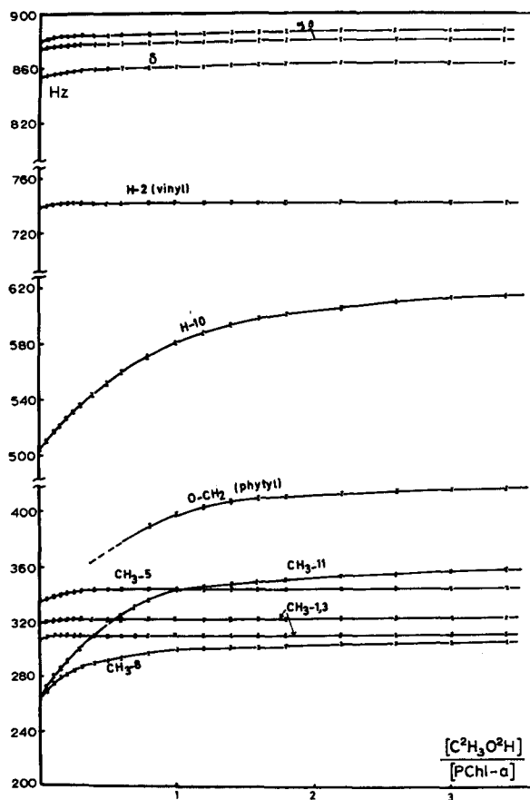
Fig. 6. Chemical shifts for ^1\text{H} magnetic resonance absorption of PChl- a ( 3.5 \cdot 10^{-2} M) in \text{C}^2\text{HCl}_3 as a function of \text{C}^2\text{H}_3\text{O}^2\text{H} /pigment concentration; chemical shifts are downfield from tetramethylsilane.
